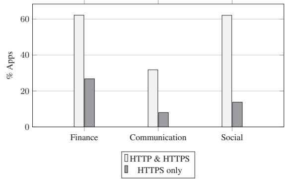
Figure 5: Empirical Statistics of Android Apps
