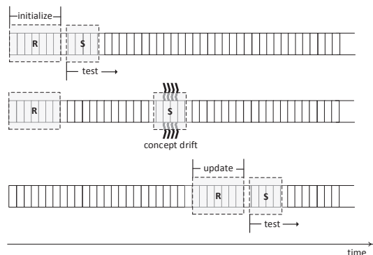
Figure 3: Illustration of ADABIND.
