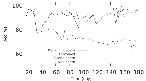
Figure 9: Adaptive Learning.
