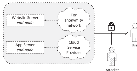
Figure 1: Illustration of website and app fingerprinting
